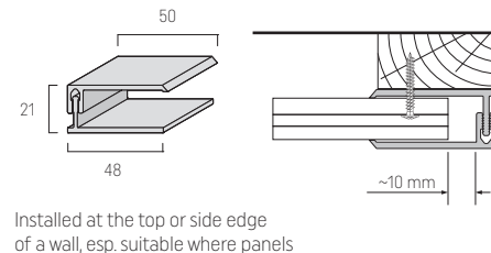
FS-252 Finishing trim, 2-piece
