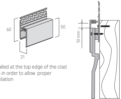
FS-262 Ventilation trim, 2-piece
