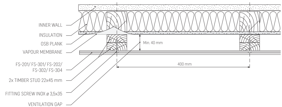
Pic. 11. Ventilation gap 40 mm required - horizontal section, see page 6
