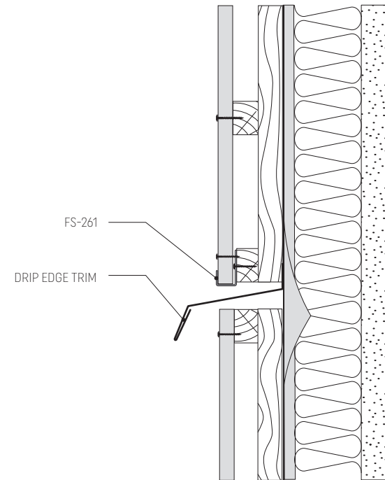
Pic. 23. Drip edge trim, detail
